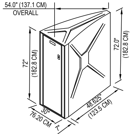
ISOMETRIC
